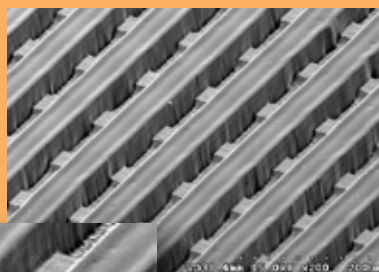
PM340, 35µm L/S Excellent Conformation on 10µm of Copper Bump
