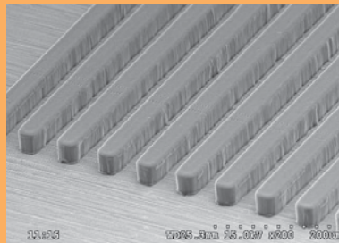
PM340, 35µm Resolution Capability
