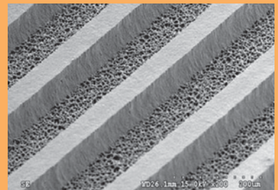
PM340, 50µm Trace
